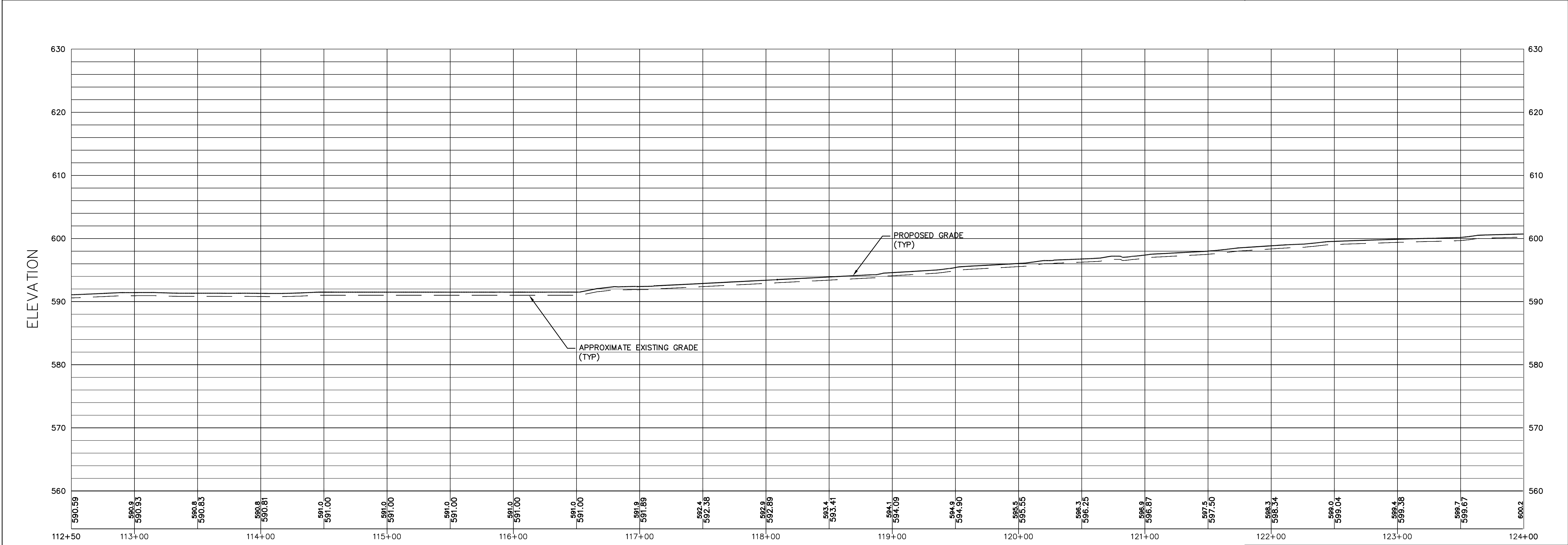
WEST KINGFIELD ROAD PROFILE HORIZONTAL SCALE 1" = 40' VERTICAL SCALE 1" = 8'
